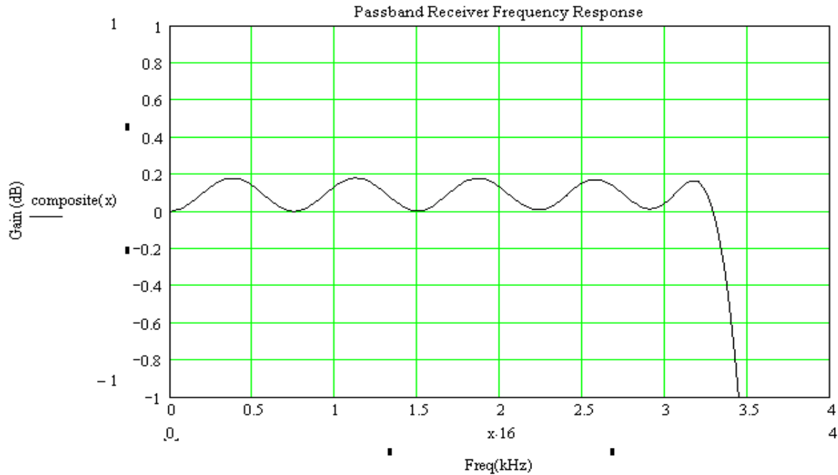
Figure 9: Rx Path Passband Response
