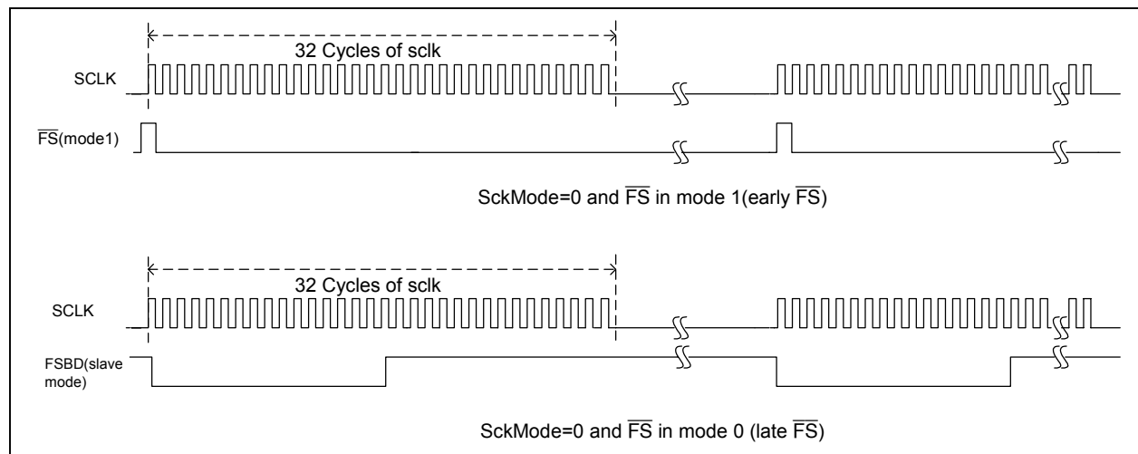
Figure 3: SCLK, FS, and FSBD
