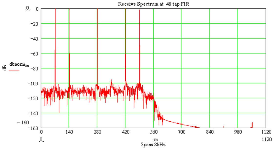
Figure 11: RXD Spectrum of 0.5kHz, 1kHz, 2kHz, 3kHz and 3.5kHz tones of Equal Amplitudes
