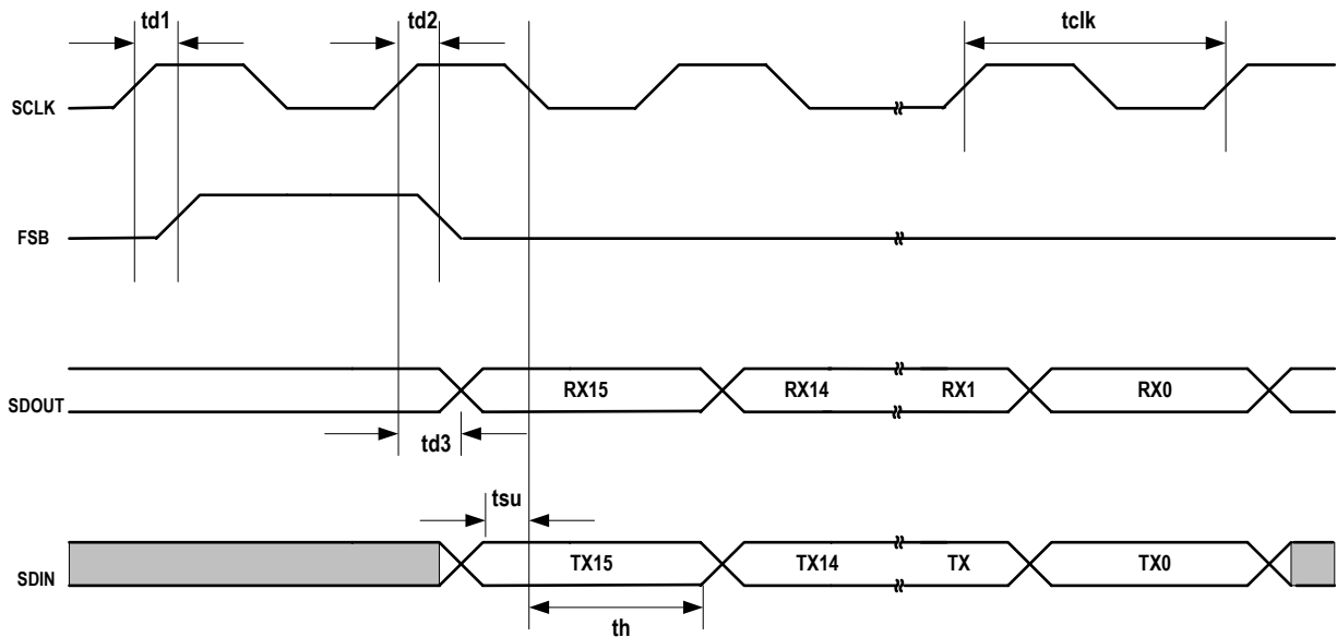
Figure 13: Serial Port Data Timing
