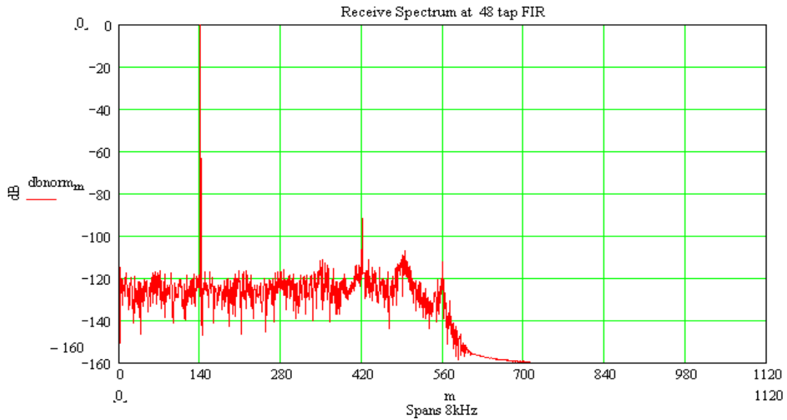
Figure 10: RXD Spectrum of 1kHz tone
