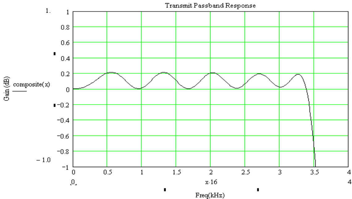
Figure 12: Frequency Response of TX Path for DC to 4kHz in band Signal
