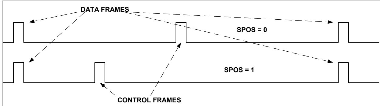
Figure 4: Control frame position vs. SPOS
