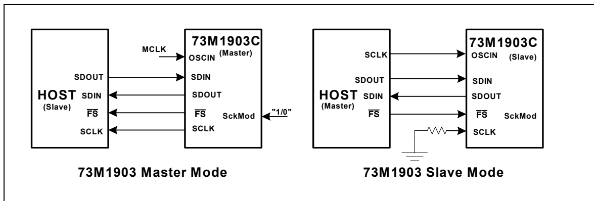
Figure 1: 73M1903C Host connection in master and slave mode
