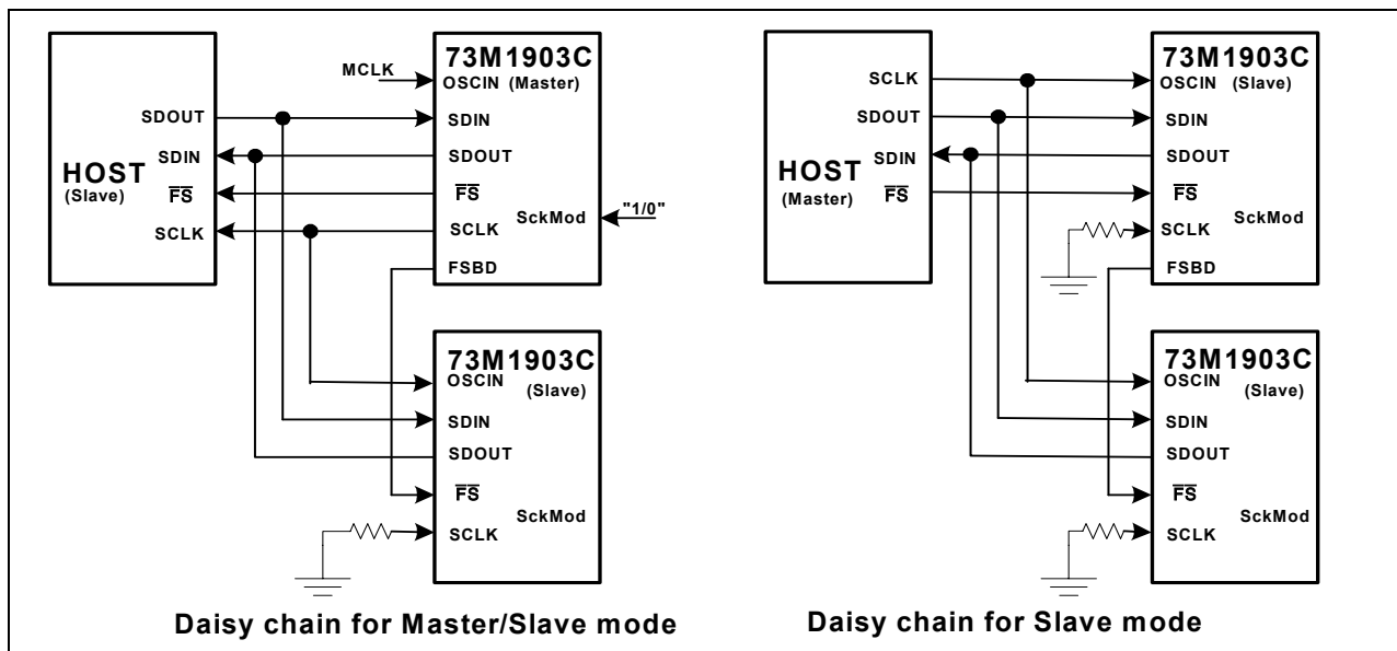
Figure 2: 73M1903C Daisy chaining for master/slave mode and slave modes
