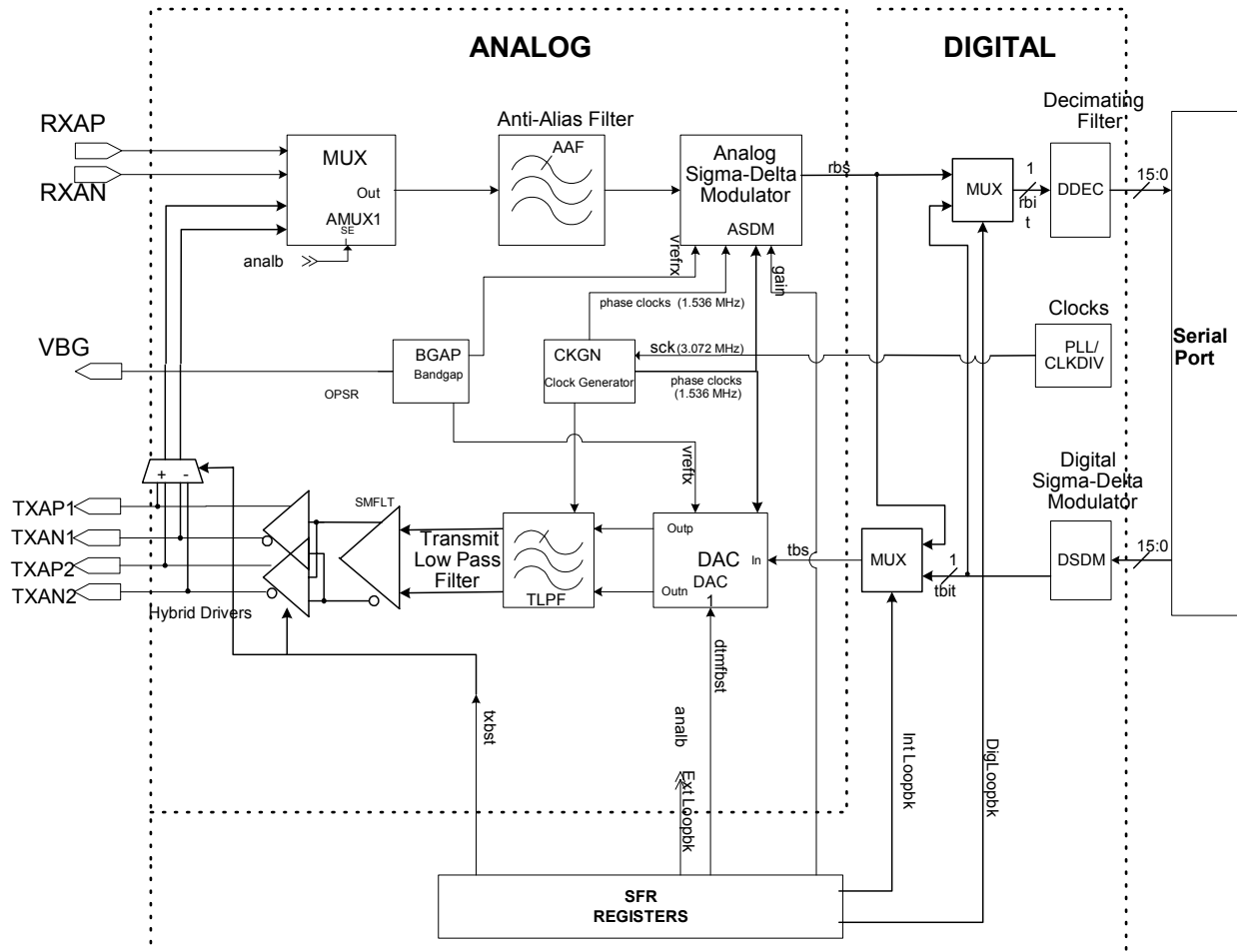
Figure 6: Analog block diagram
