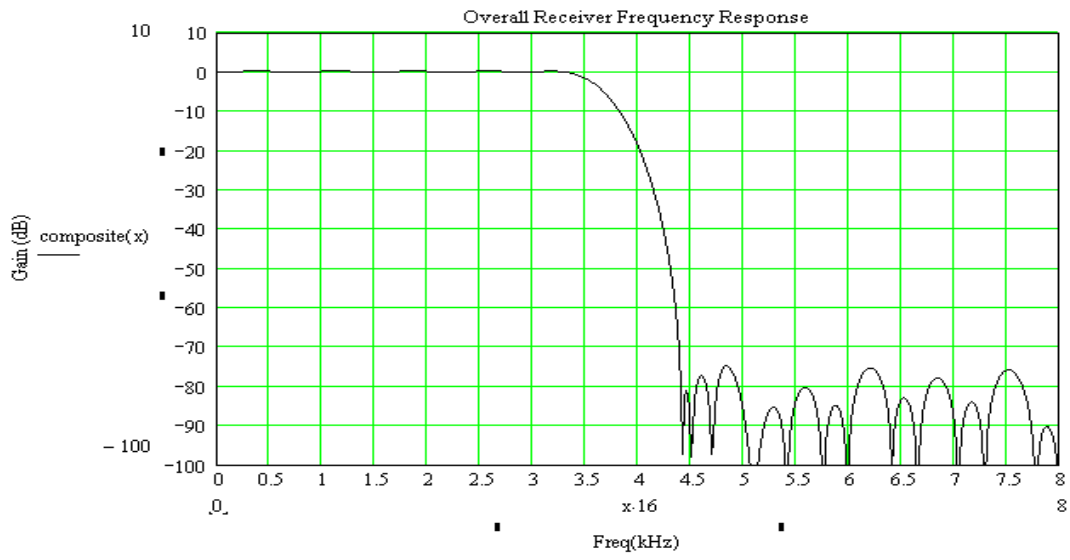
Figure 8: Overall Receiver Frequency Response
