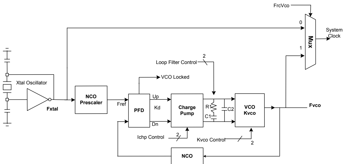
Figure 7: Clock Generation
