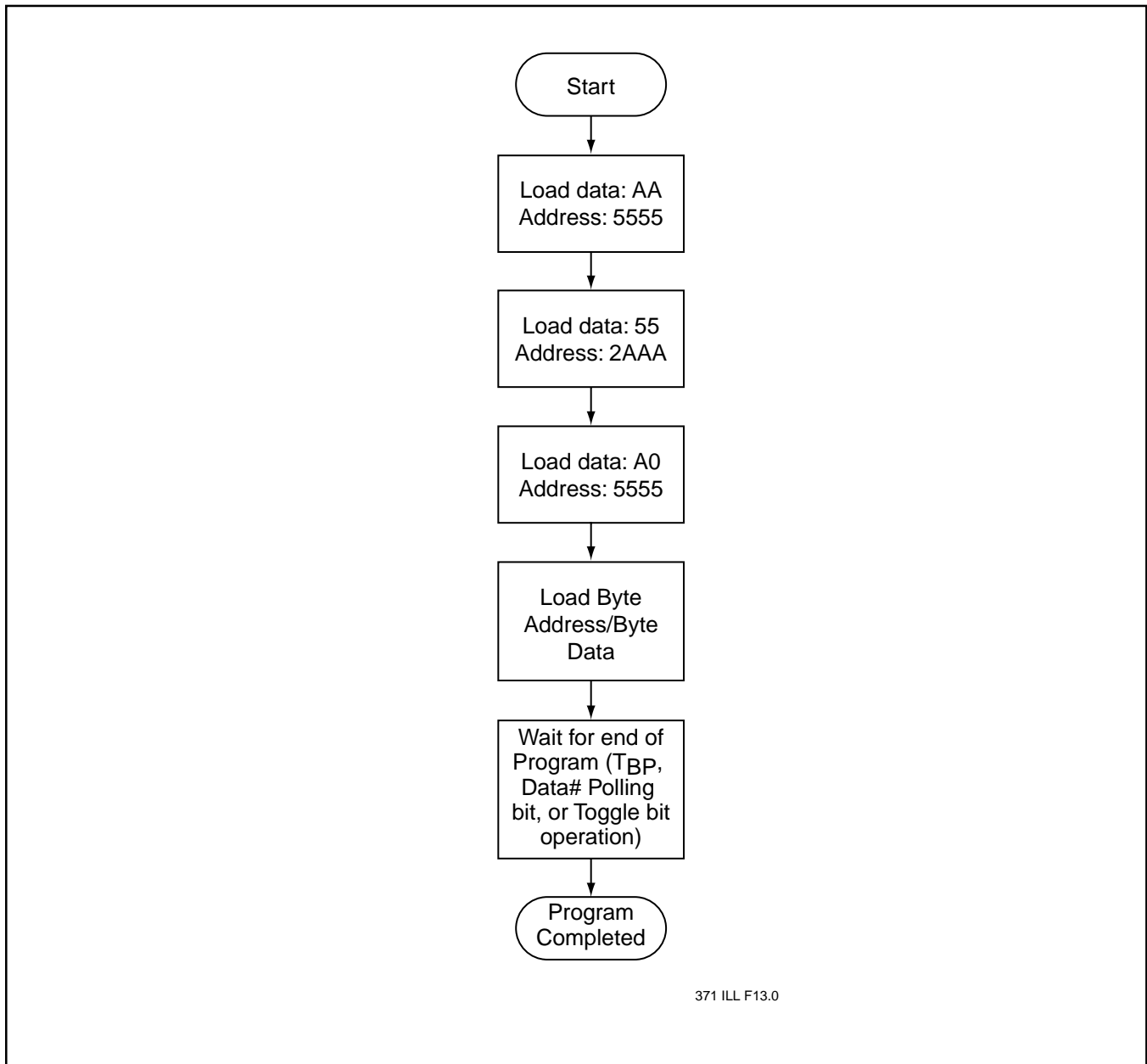
FIGURE 16: BYTE-PROGRAM ALGORITHM
