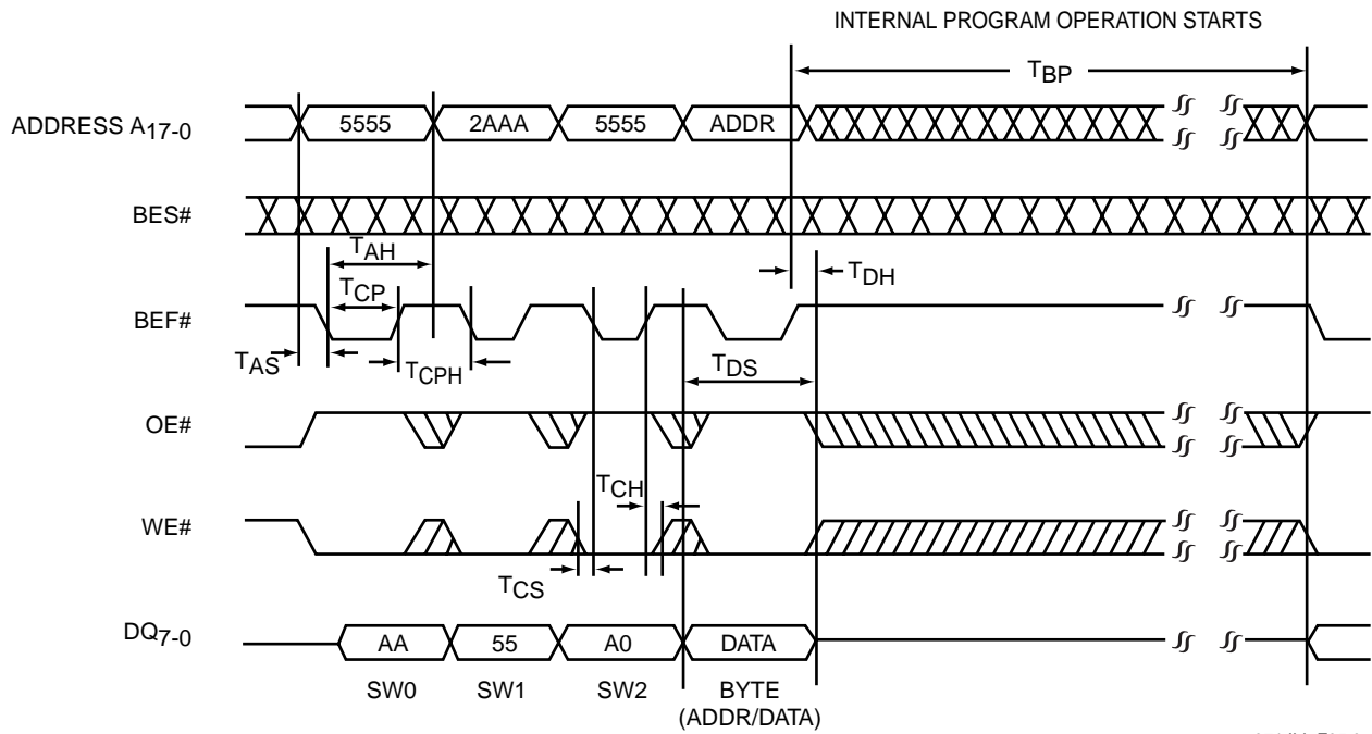
FIGURE 6: FLASH BEF# CONTROLLED PROGRAM CYCLE TIMING DIAGRAM
