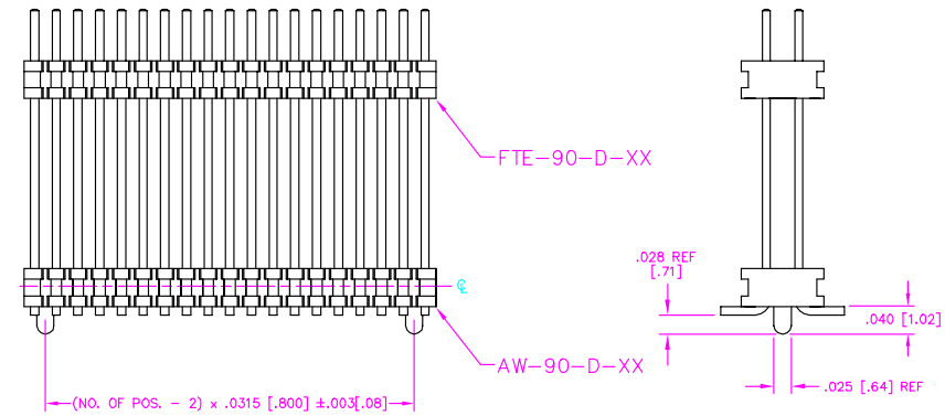
FIG. 5 (DIFFERENT AS SHOWN, OTHERWISE SAME AS FIG. 1) -A OPTION MOLDED (4 POS MIN)
