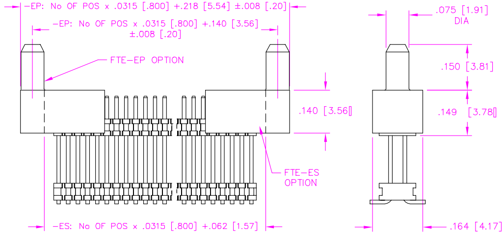
FIG. 4 POST HEIGHT MUST BE .075 [1.91] (DIFFERENT AS SHOWN, OTHERWISE SAME AS FIG. 1)
