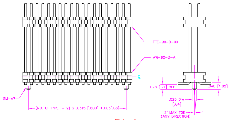
FIG. 6 (DIFFERENT AS SHOWN, OTHERWISE SAME AS FIG. 1) -A OPTION (STAKED) (7 POS MIN)
