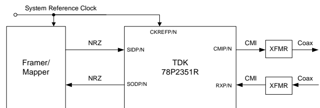
Figure 2: Synchronous
